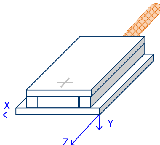
Figure 4. Reference Cartesian coordinate system of the SENIS I3A-03C Hall probe. NOTE: The Probe case of the C-Vacuum probe is open on the front side.
