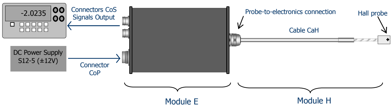
Figure 1. Typical measurement setup with a SENIS magnetic-field-to-voltage transducer with integrated 3-axis Hall probe (module H) and electronics (module E, encapsulated in the box type B)
