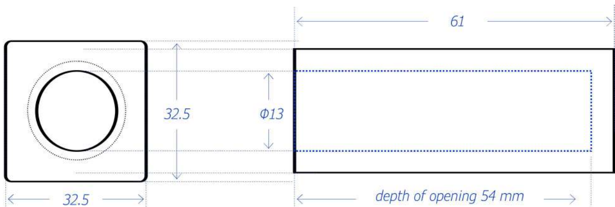
Figure 2. Dimensional drawing of the Zero Gauss chamber ZG-12-LN. All dimensions are in millimeters (mm).
