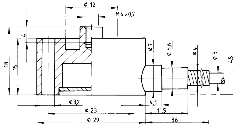
Dimensional drawing – Measuring range ≤ 0 ... 2000 N | 450.0 lbs
