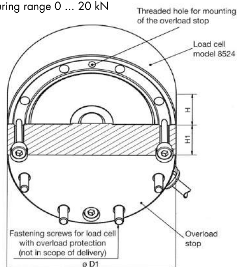
Example for measuring range 0 ... 20 kN
