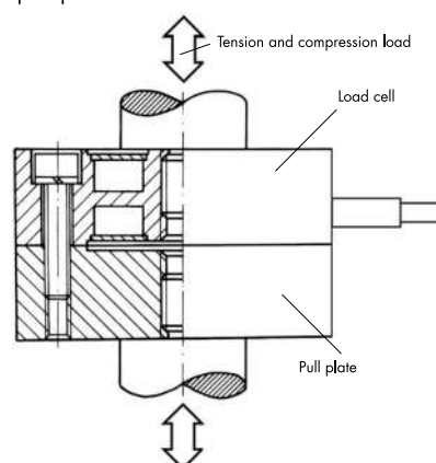
Sensor with pull plate
